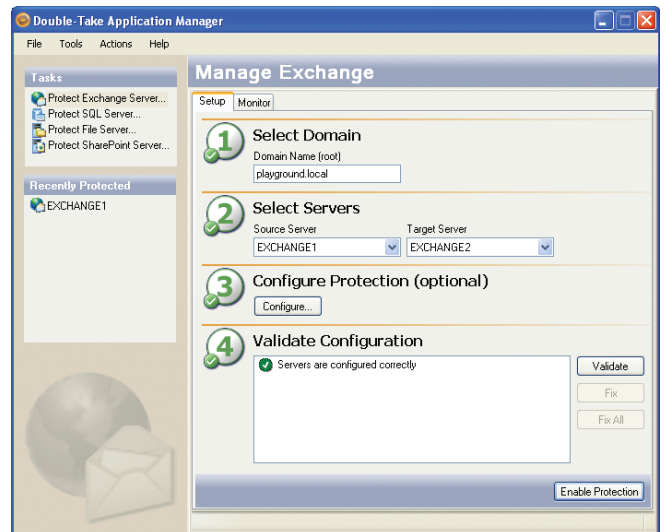
Figure 2: Double-Take Availability Application Manager
